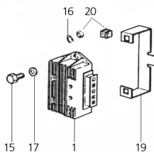
Vespa 100/S/PK 50-125
